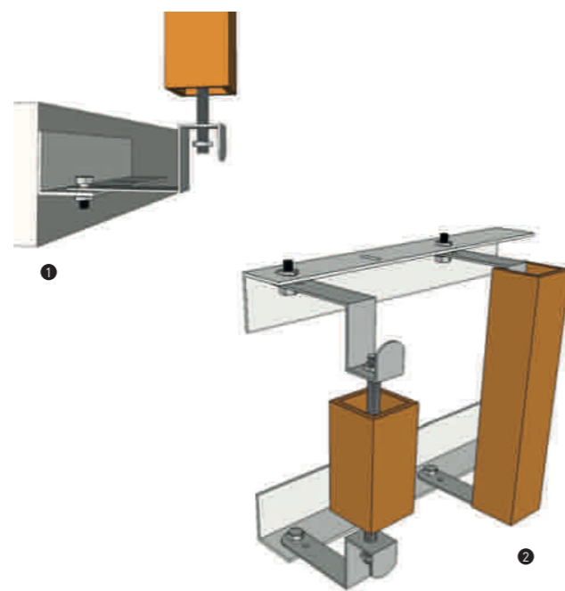
HOOK SYSTEM
