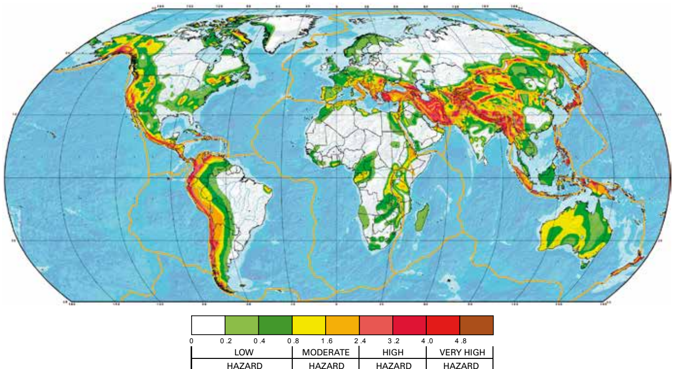
Seismic hazard map – zones worldwide
