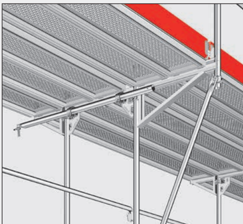
Wall tie with two plate couplers
