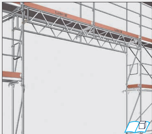
Example: SpeedyScaf lattice beam 5.14 m, covered scaffolding (special diagonal guidance)
