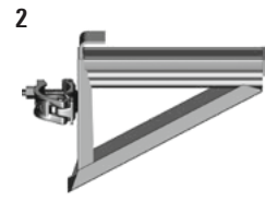
The console bracket, 0.36 m for decks, 0.32 m
