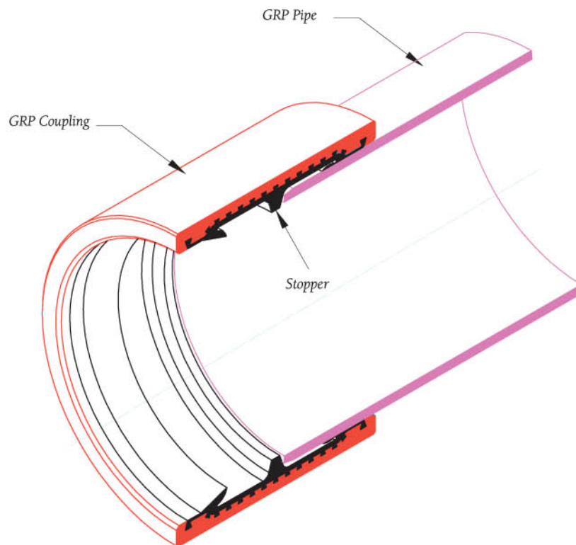
Figure 13 : Coupling section
