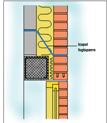
Facadelukninger
