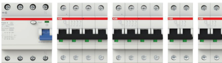
C3-2 HPFI-A 40A30mA + 2x4P 16A-C + 2x2P 10A-C
