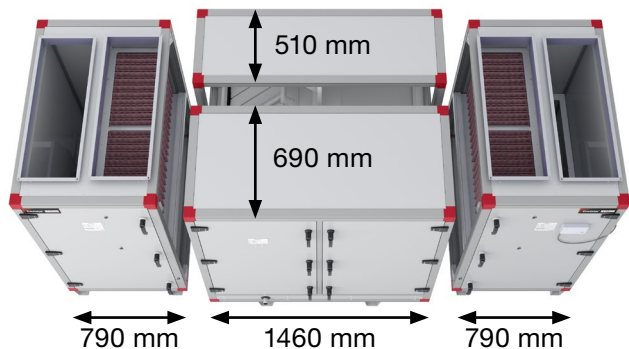
Envistar Top size 12 with split counter-flow exchanger.
